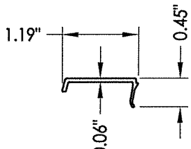
3 GLAZING BEAD 8571-356-D58
