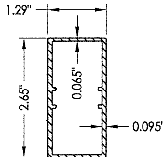
10 REINFORCEMENT 356-A54-55
