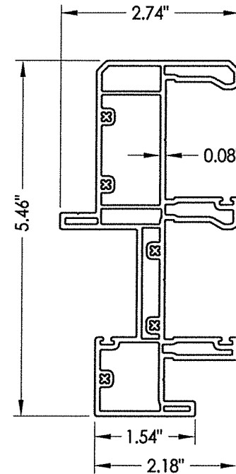
21 MULLION 356-A61
