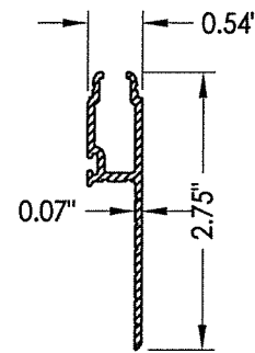
17 HIGH DAM 356-A51-DP70
